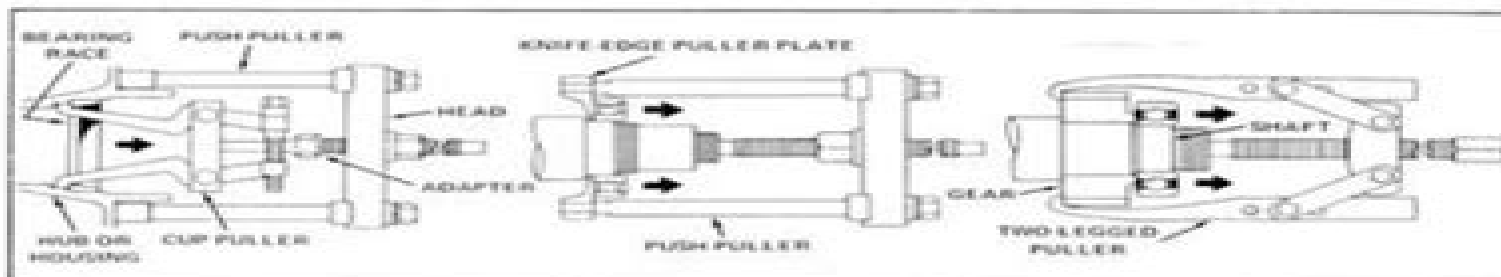
Figure 2-2. Correct Puller Methods
