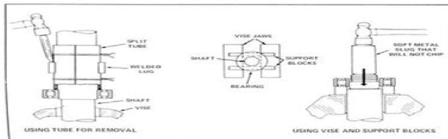
Figure 2-3. Removing Bearings with a Hammer
