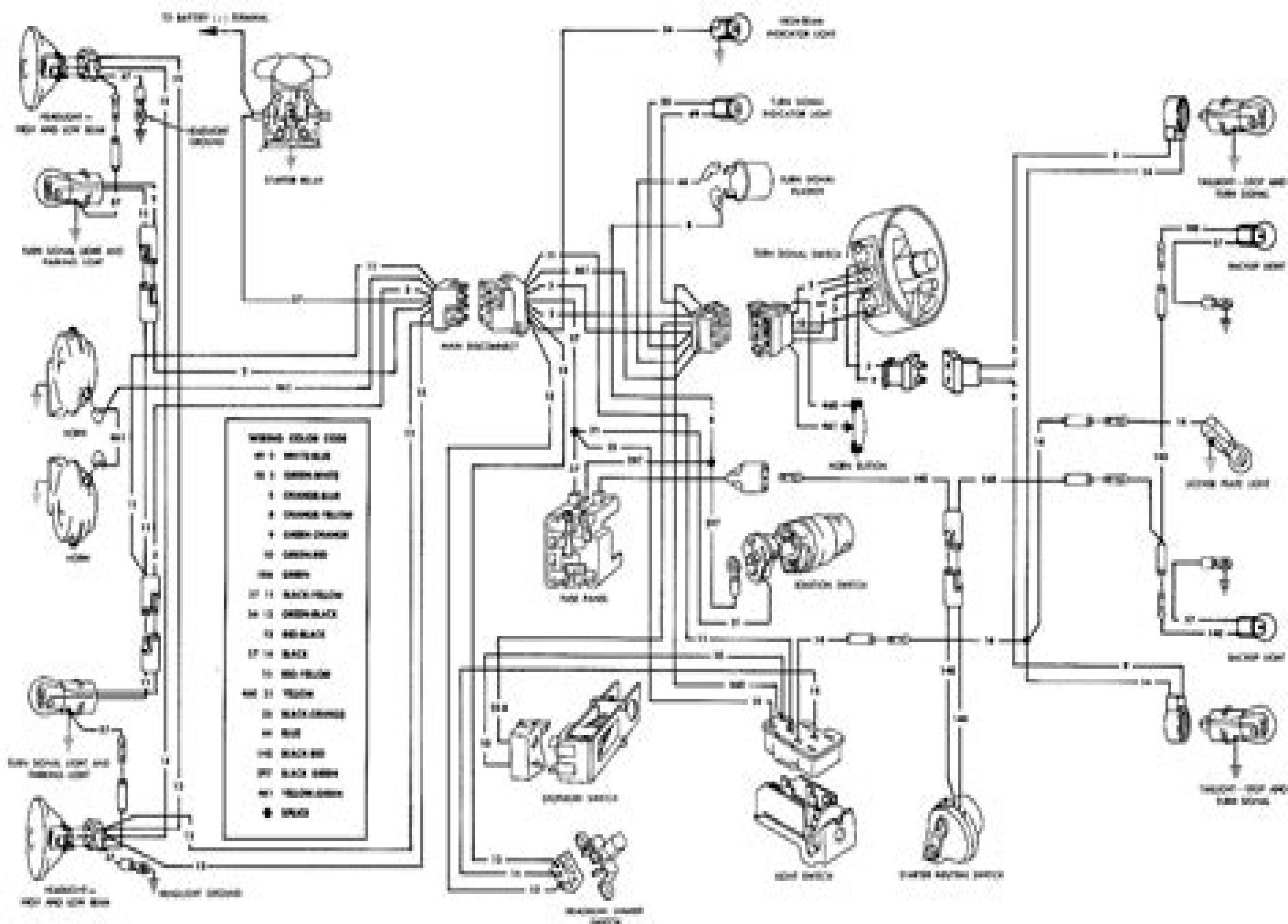
1965 MUSTANG EXTERIOR LIGHTING, TURN SIGNALS AND HORNS
