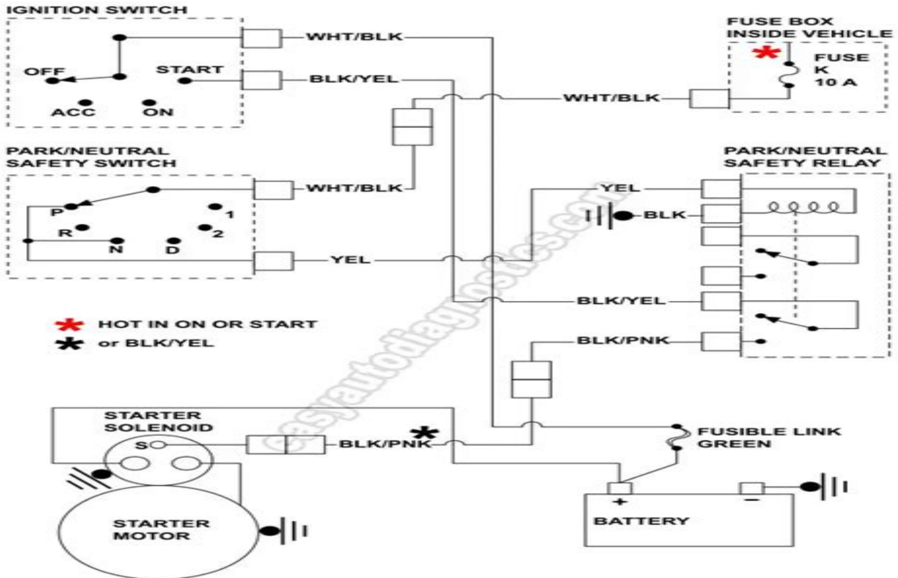
STARTER MOTOR WIRING DIAGRAM (AT) (1992-1994 2.4L PICKUP D21)
