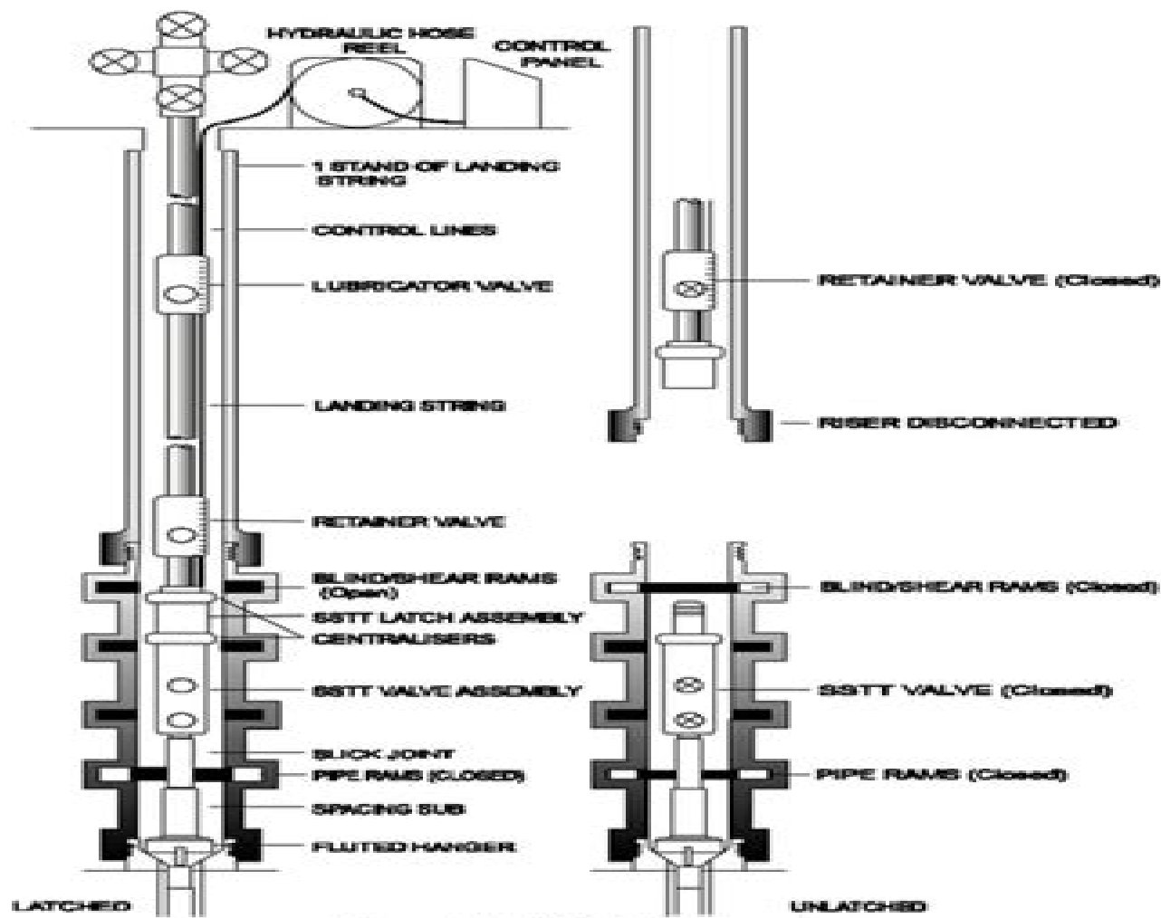
Figure 5.A - SSTS Arrangement
