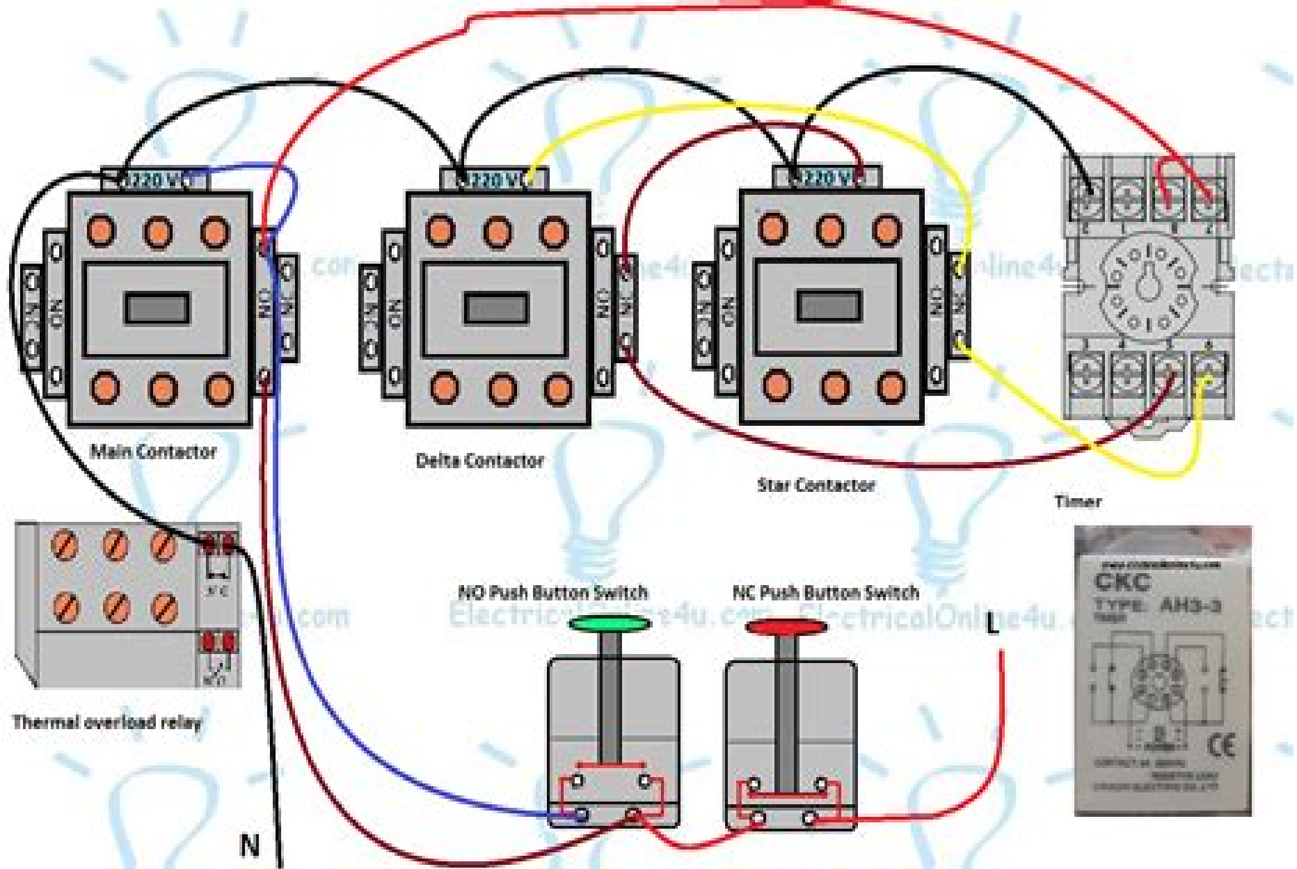
Star Delta Starter Control Wiring Diagram With Timer
