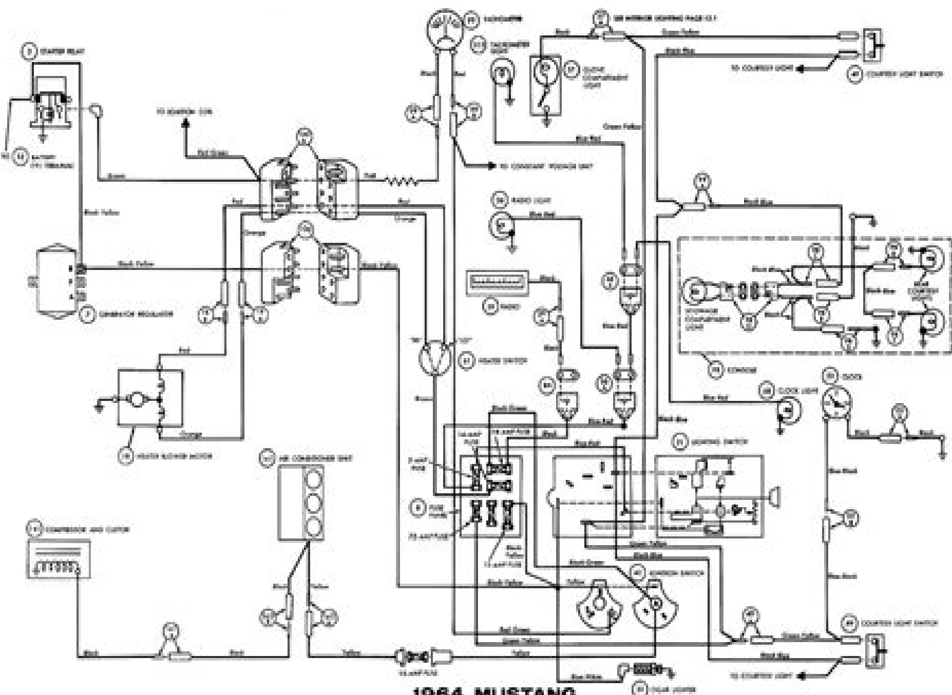
1964 MUSTANG ACCESSORIES SCHEMATIC
