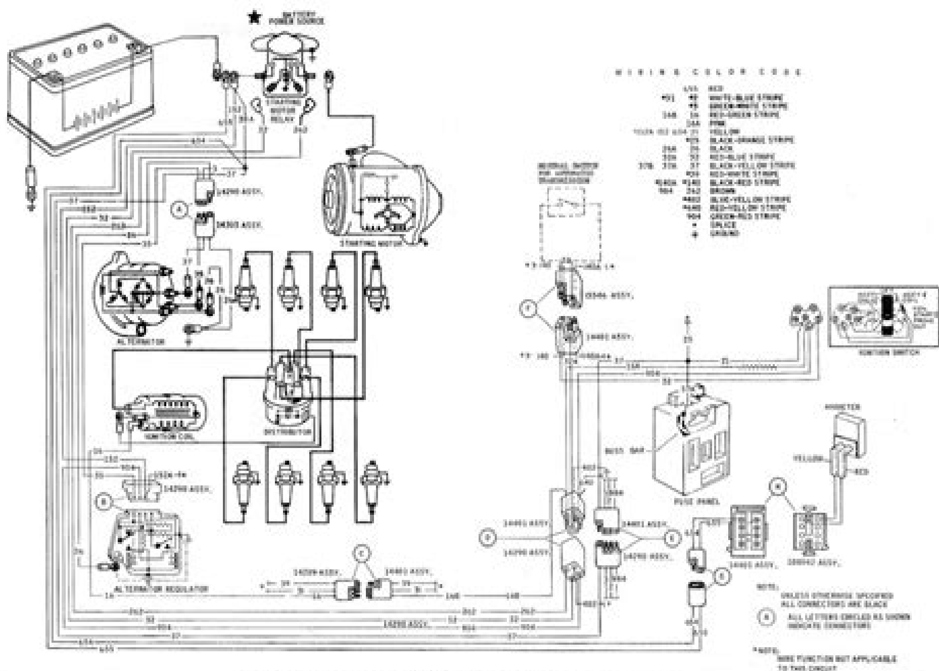
1968 MUSTANG IGNITION, STARTING AND CHARGING
