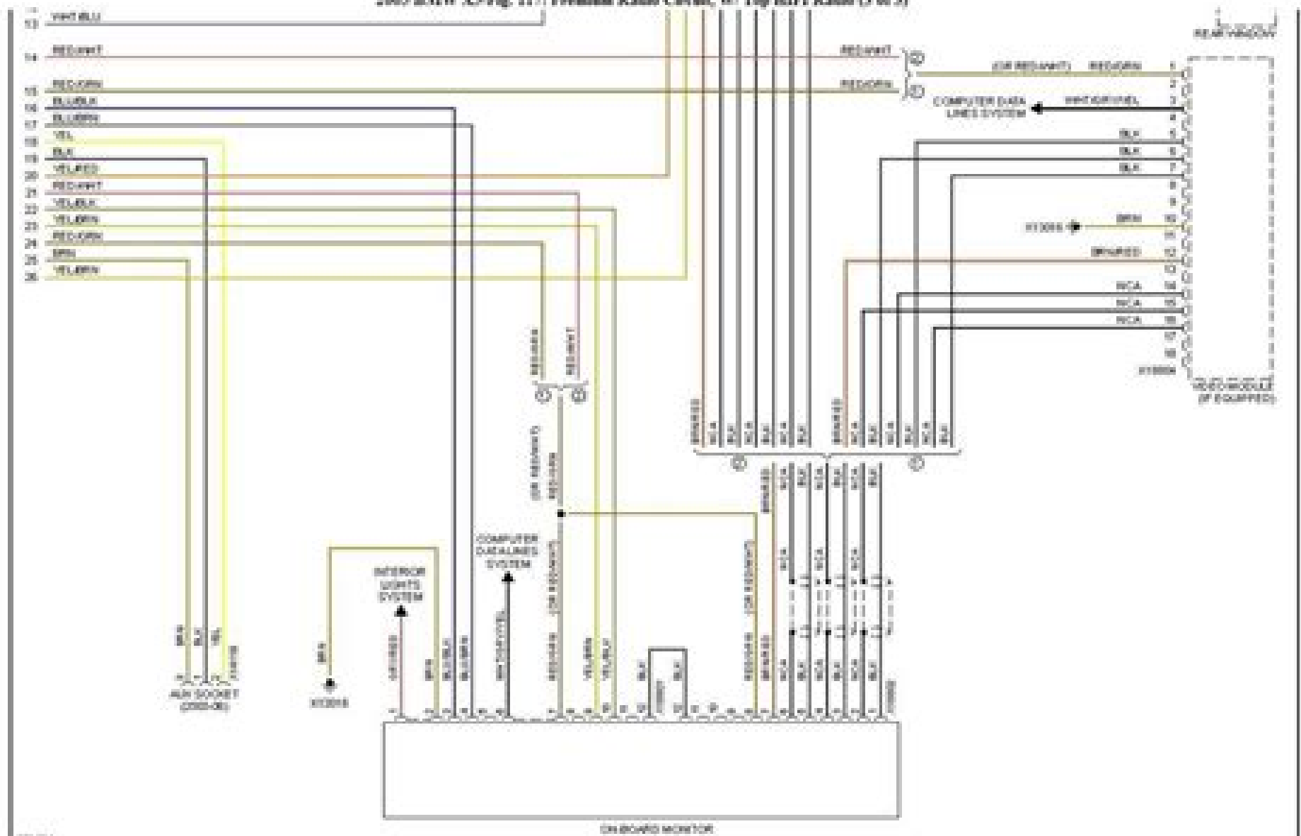
2005 BMW X5- Fig. 117: Premium Radio Circuit, W/ Top RF1 Radio (3 of 3)
