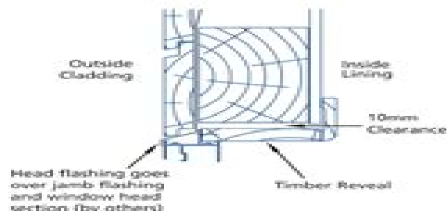
TIMBER FRAME HEAD
