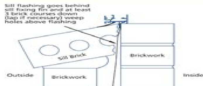
CAVITY BRICK SILL
