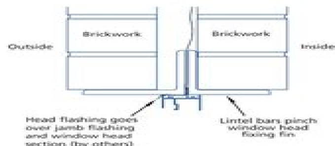
CAVITY BRICK HEAD
