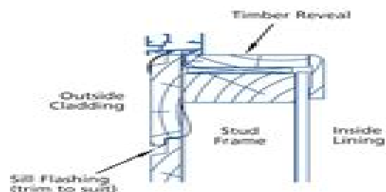
TIMBER FRAME SILL
