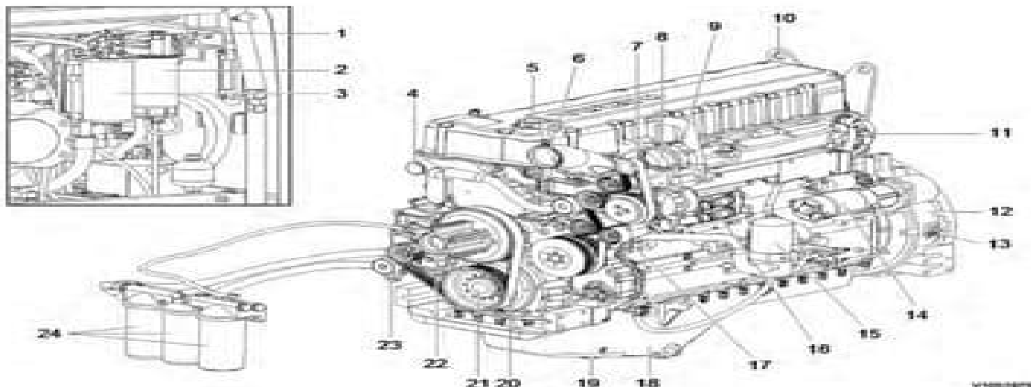
Figure 1 Engine, structure
