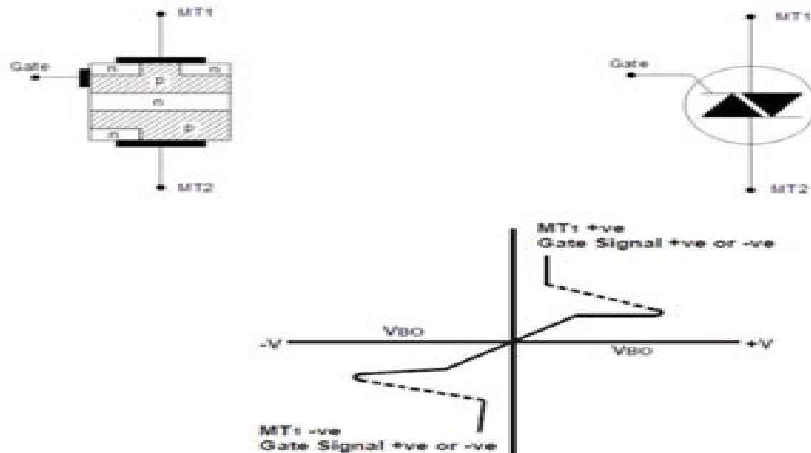
Fig. 1 Construction, Symbol and Characteristics
