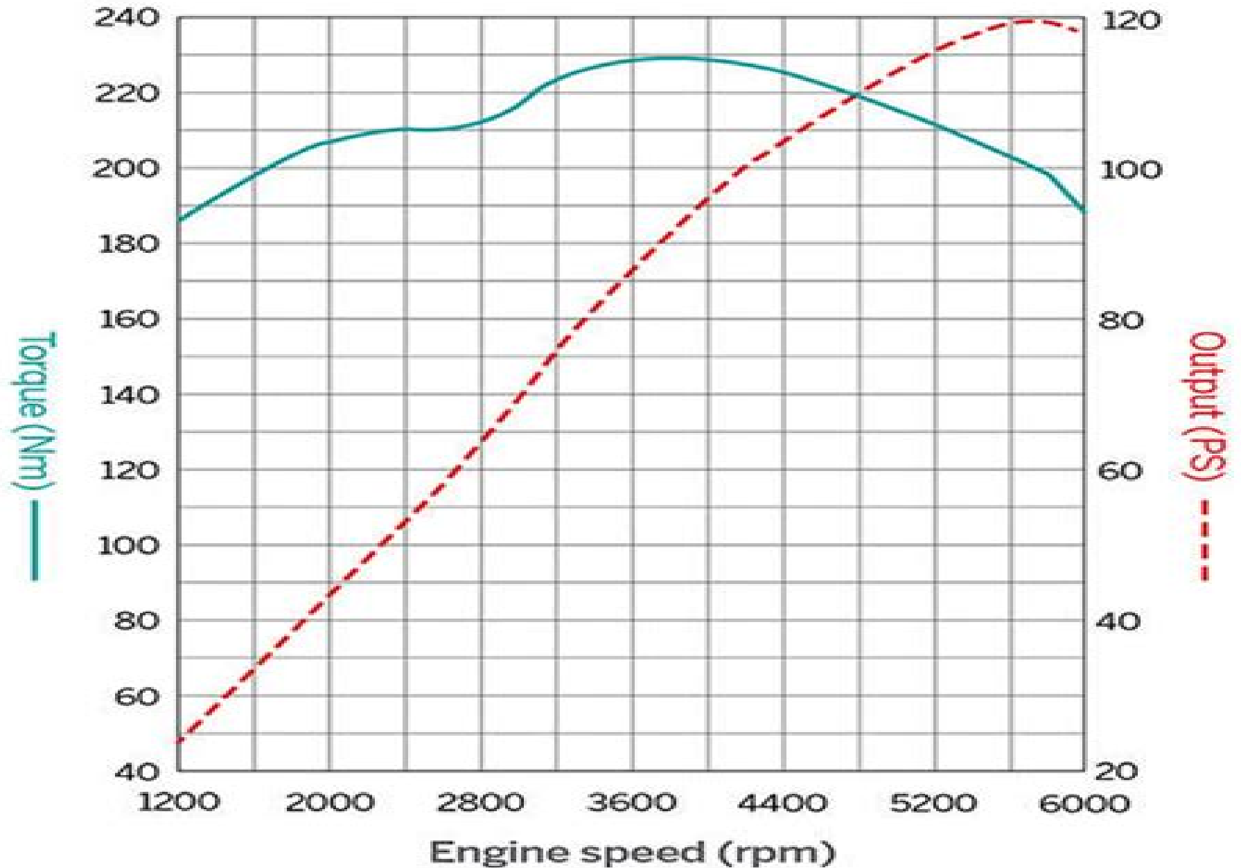
A sample engine performance curve
