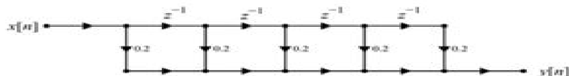
FIGURE 2.15: Block diagram of a 5-point moving average filter.
