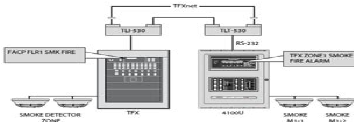
Figure 1 TFXi Functional Overview (4100U Shown)
