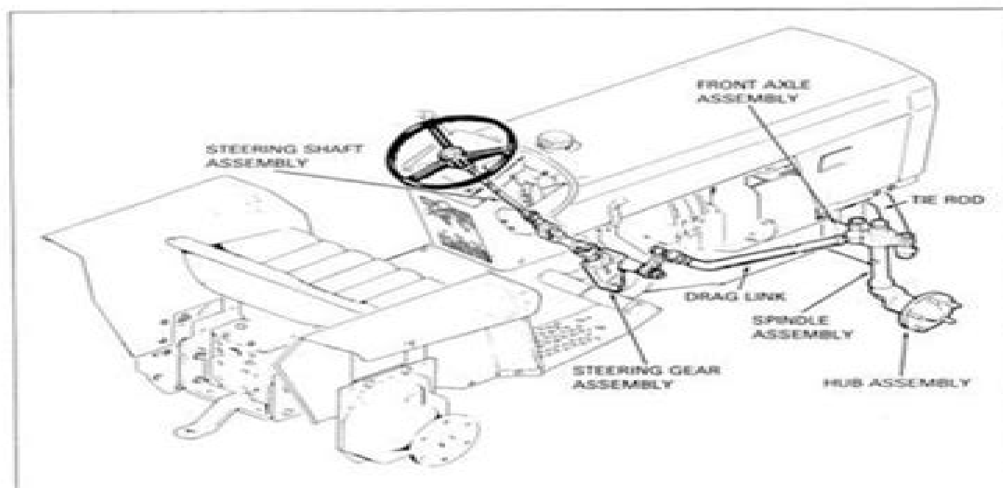
Figure 45. Steering and Front Axle Assemblies
