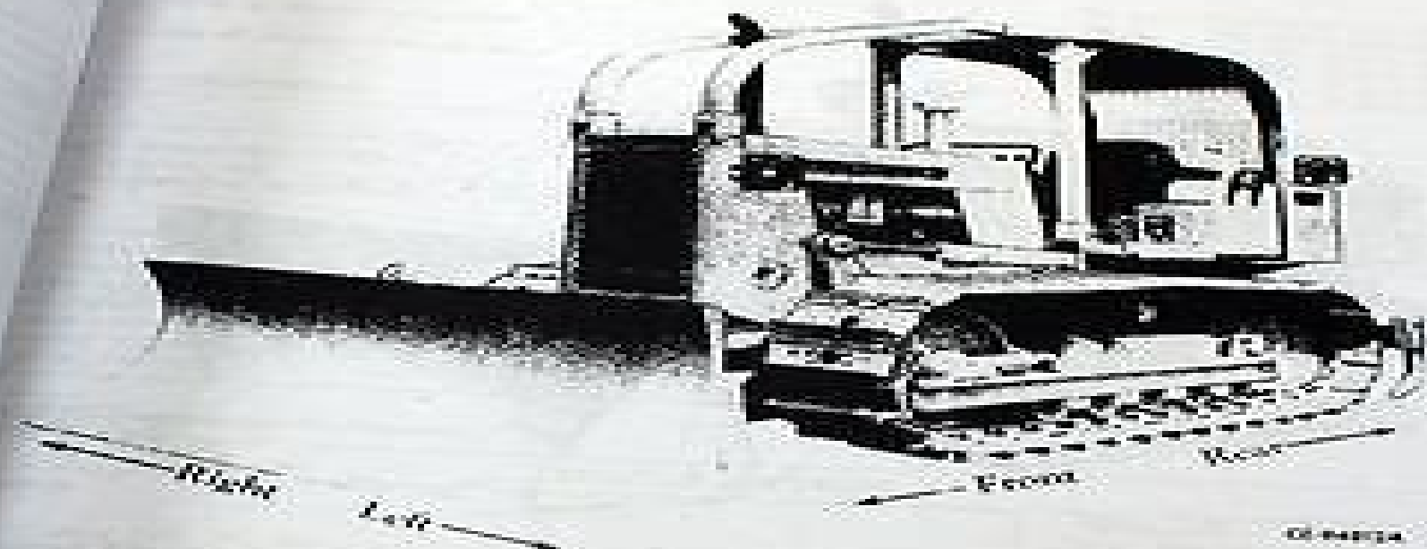
FIGURE 1 TO 8 SERIES E Single Arm Drive with Rigid CTO 8 SERIES C, TO 7 SERIES C and E Similar
