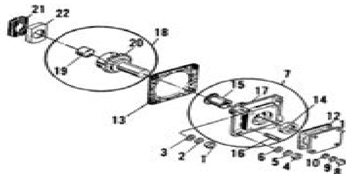
FIGURE 4-5. MAGNETO & ACCESSORY DRIVES.
