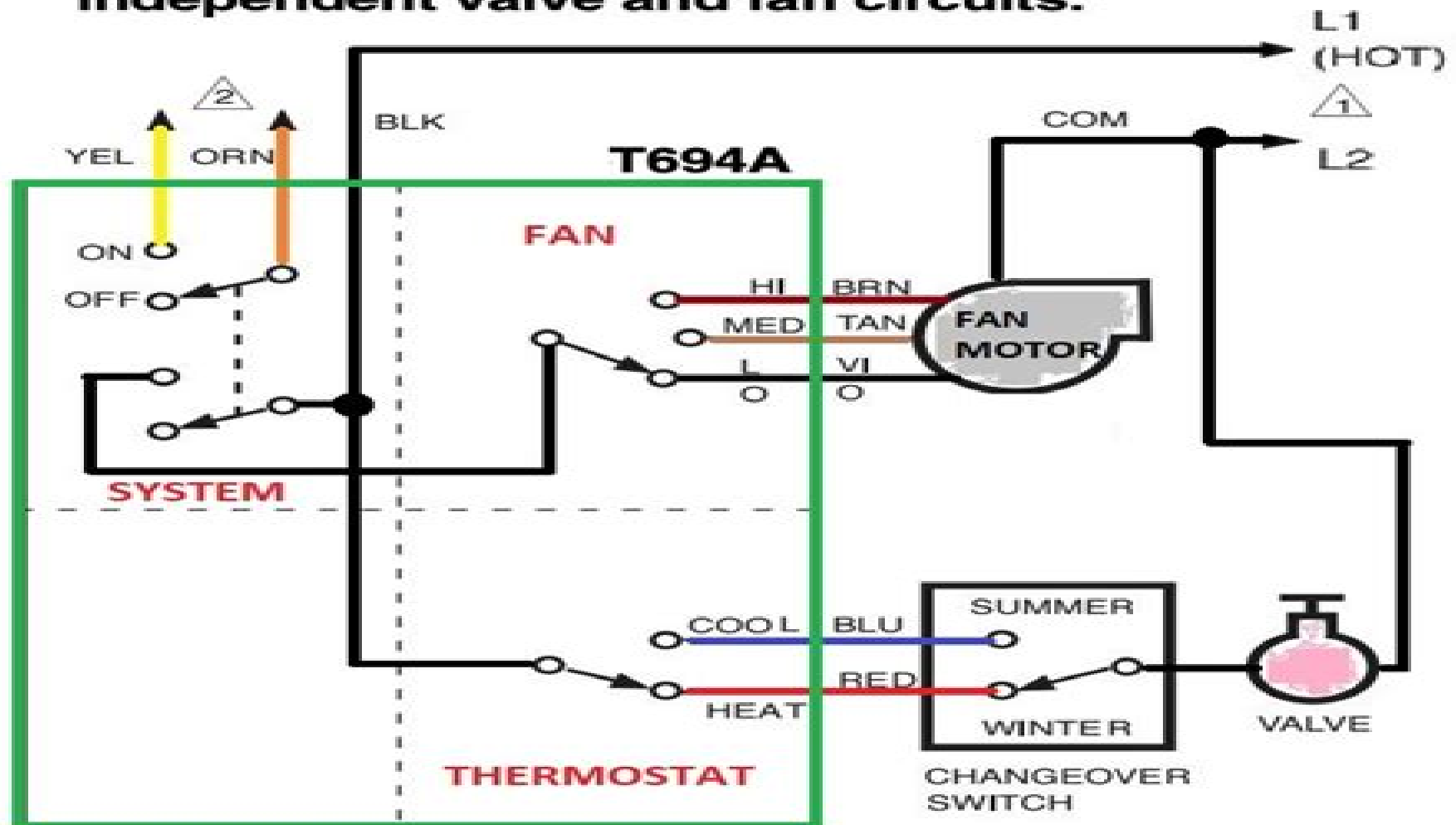
Fig. 6—T694A in heating-cooling system with independent valve and fan circuits.
